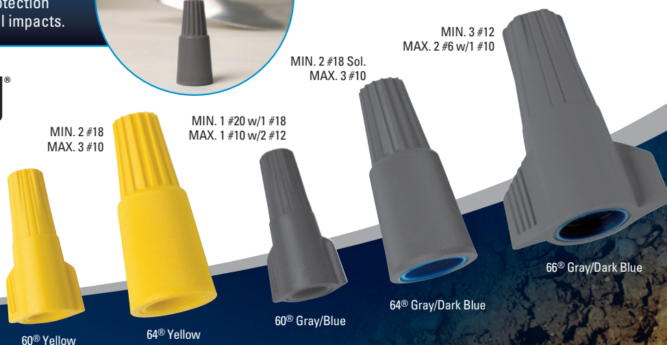
UnderGround™/MudBug® Wire Connector:
